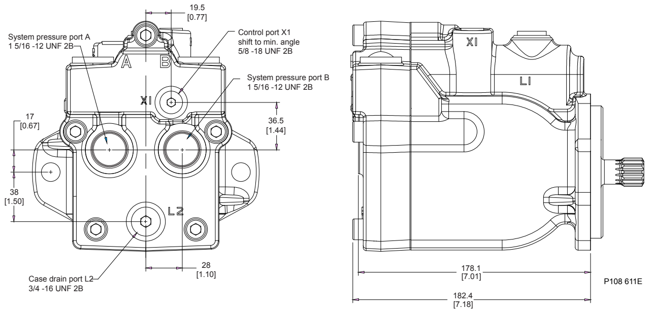
Axial ports without loop flushing
