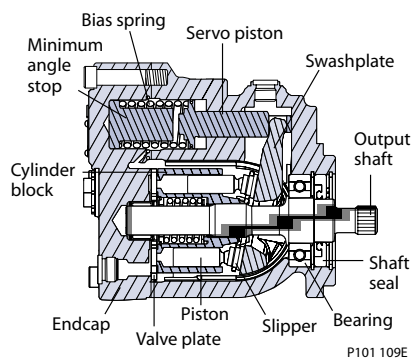
Cross section, cartridge mount
