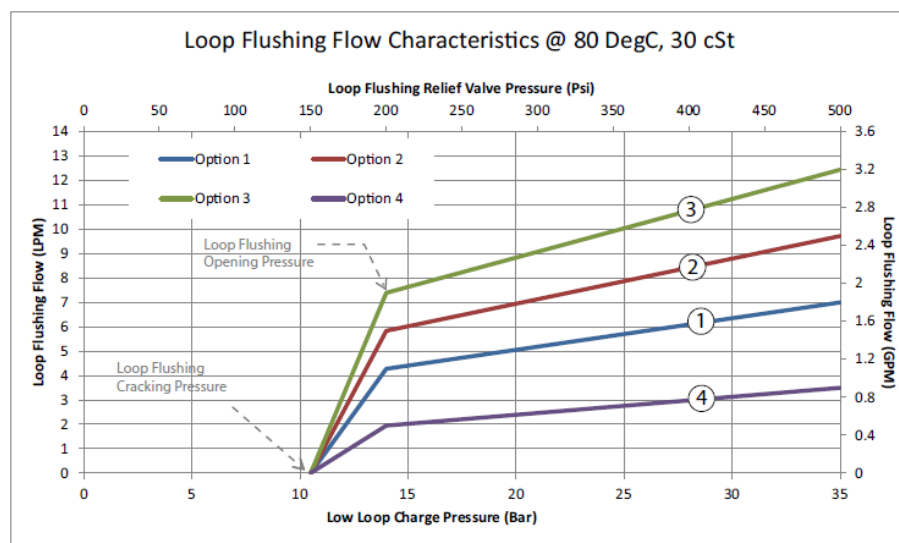
Loop Flushing flow
