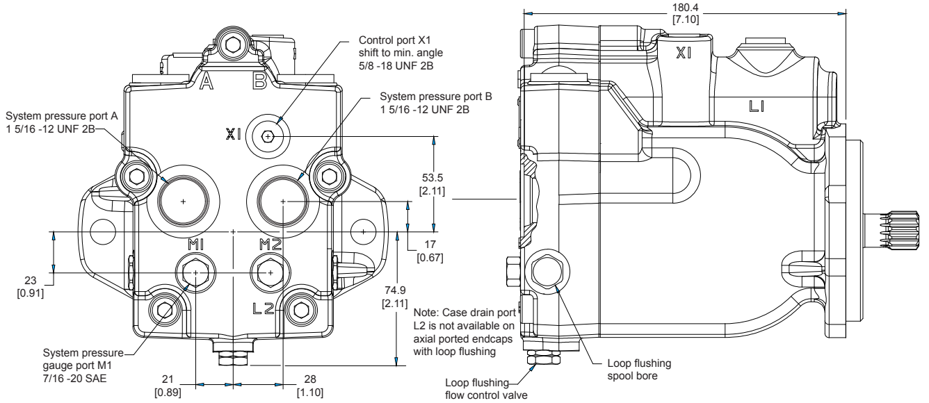
Axial ports with loop flushing
