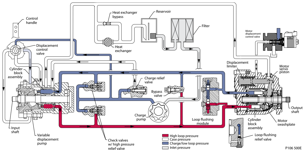
Pictorial system diagram
