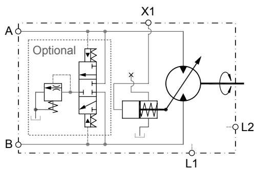
Cartridge motor - single line control
