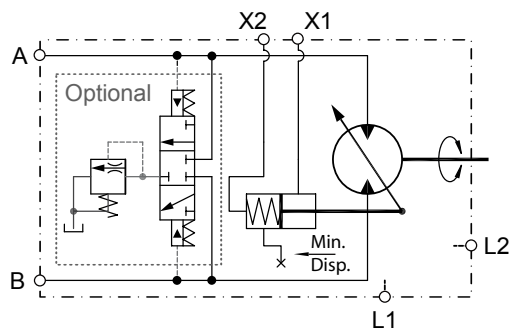
SAE motor - single or two line control
