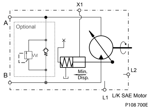
Anti-Cavitation Valve, Port B High Pressure
