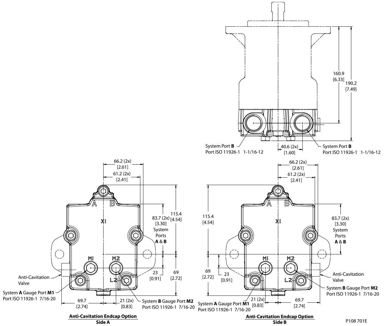
Radial ports with Anti-cavitation valve
