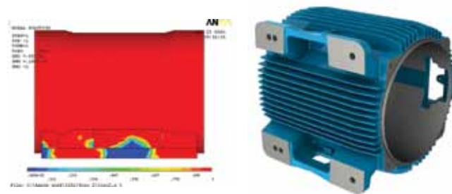
Figure 4 – Solid feet
