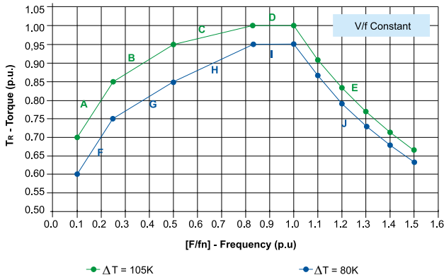
Figure 32 – Derating curve for constant flux
