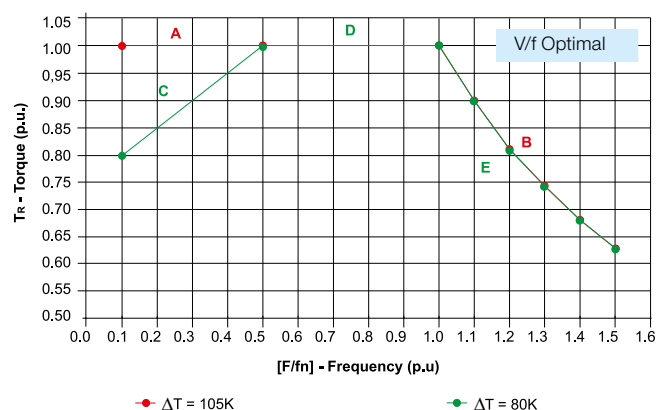
Figure 33 – Derating curve for optimal flux®
