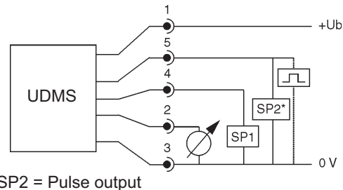
Connection diagram B (2 switching outputs, 1 analog output)
