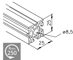
Profile mk 2025.31
