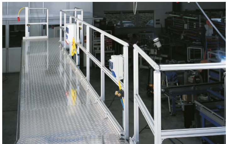
Guardrail posts built from mk profile technology can be used to attach various components, e.g. electronics supply equipment
