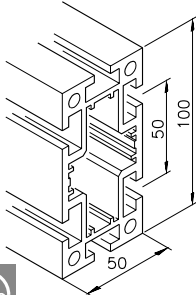
Profile mk 2004
