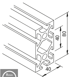
Profile mk 2040.02
