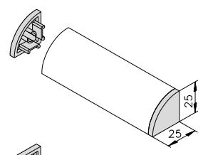
End cap for mk 2550.37 25.50.8004 Black
