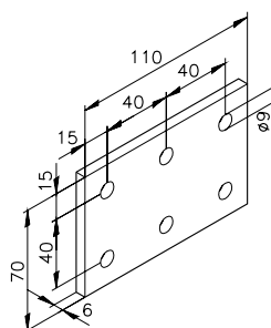
Connection plate 40/2 50.05.0060
