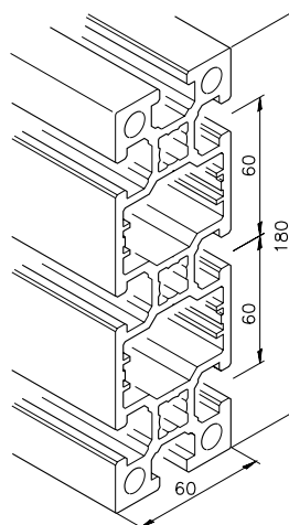
Profile mk 2060.03
