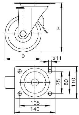
Swivel caster (B) with locking device
