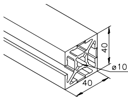
Profile mk 2040.95
