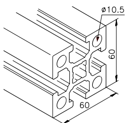
Profile mk 2060.01
