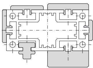
Series 50 fastening example
