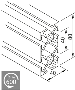
Profile mk 2040.41 (light duty)
