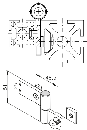
Hinge combination 25-1/40-1
