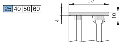
Dimensional sketch
