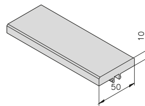
Wear strip mk 1070 22.70.2000
