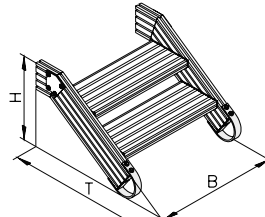
Stairs 35° B02.31.006
