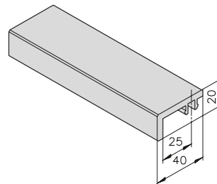
Wear strip mk 1008 22.08.2000
