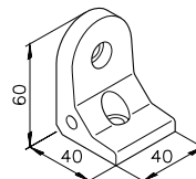
Angle F40/R 82.40.0805
