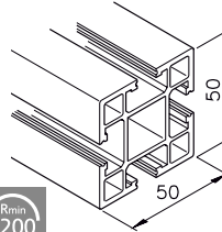
Profile mk 1014 (light duty)
