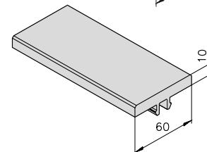
Wear strip mk 1060.62 21.62.2000
