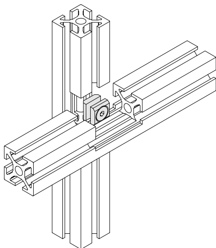
Fastening example for B51.03.056
