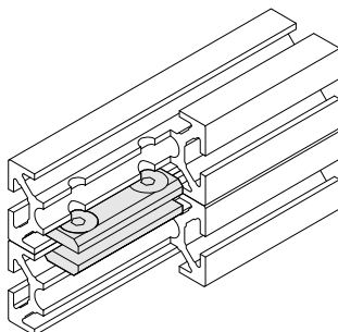
Fastening example for B51.03.056
