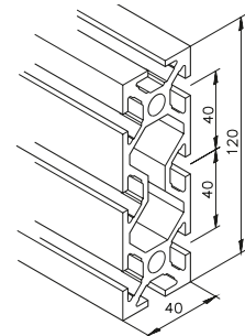
Profile mk 2040.05
