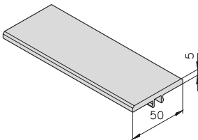
Wear strip mk 1001 22.01.2000
