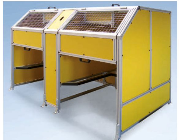
Custom guarding with lifting swing door operated by pneumatic springs
