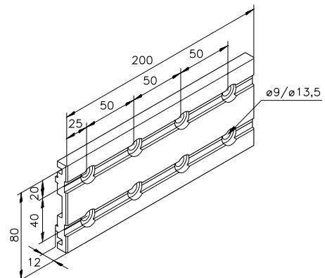
Profile 3856 3856BD0200
