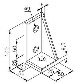
Angle bracket 1 31.00.0001
