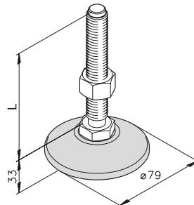
Levelling foot ø 79 M12 B67.02.001
