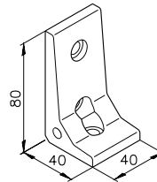
25 40 50 60 Angle F40 82.40.0802
