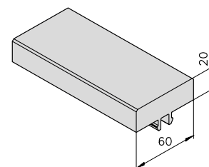
Wear strip mk 1060.64 21.64.2000
