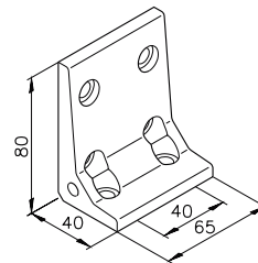
Angle F65 82.40.0804
