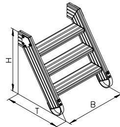
Stairs 55° B02.31.008
