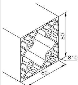
Profile mk 2040.109
