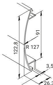
Profile mk 2040.44
