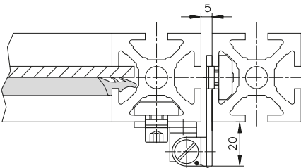
Ball latch for 5 mm door gap, B68.02.101
