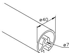
Profile mk 2040.16
