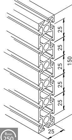
Profile mk 25.04
