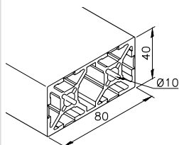
Profile mk 2040.104
