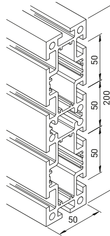
Profile mk 2008
