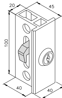
External double-bit lock DIN right B68.02.017
