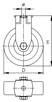
Fixed casters (A)
