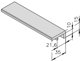
Wear strip mk 1040.05 21.05.2000
