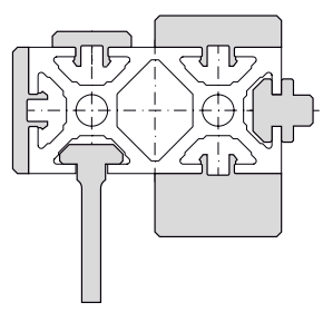
Series 40 fastening example
