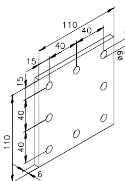
Connection plate 40/4 50.05.0062
