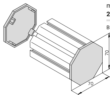
End cap for mk 2550.38 25.50.8005 Black
