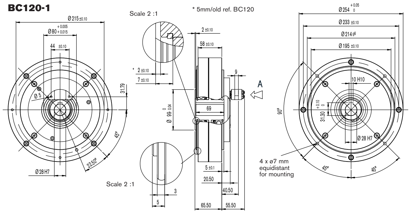
VIEW A - Brushes holder
