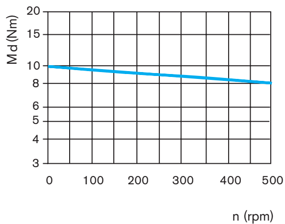
Brake torque
