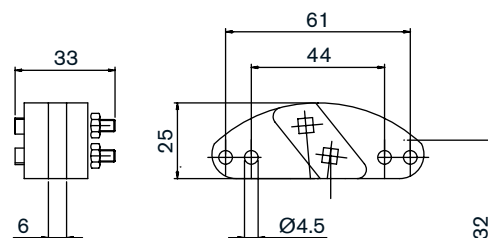
VIEW A - Brushes holder
